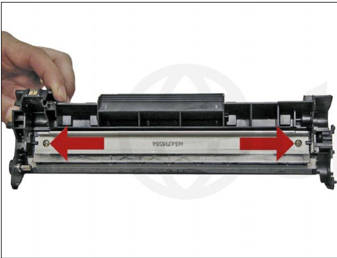
6. Remove the two screws and the wiper blade.
