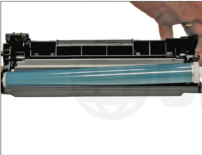
4. On the waste/drum section, lift the drum up from the gear side. Twist and remove from the hopper.
