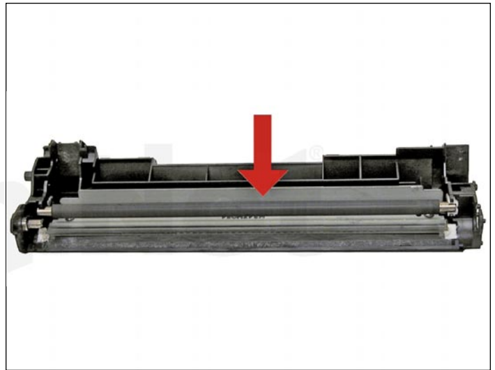
5. Remove the PCR and clean with your standard PCR cleaner.
